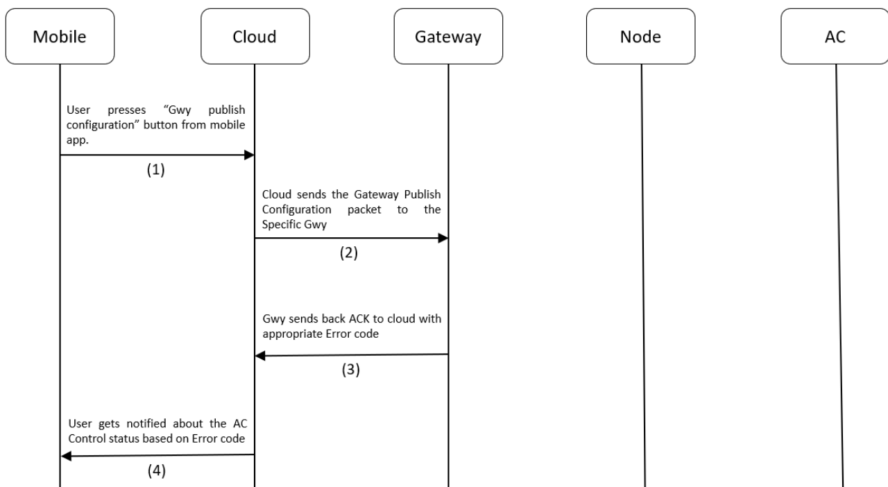
Figure 4.14 Gateway Publish Configuration Process flow
