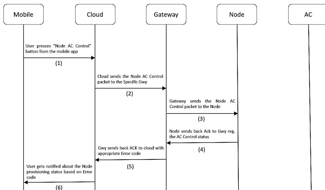
Figure 4.24 Node AC Control Process flow
