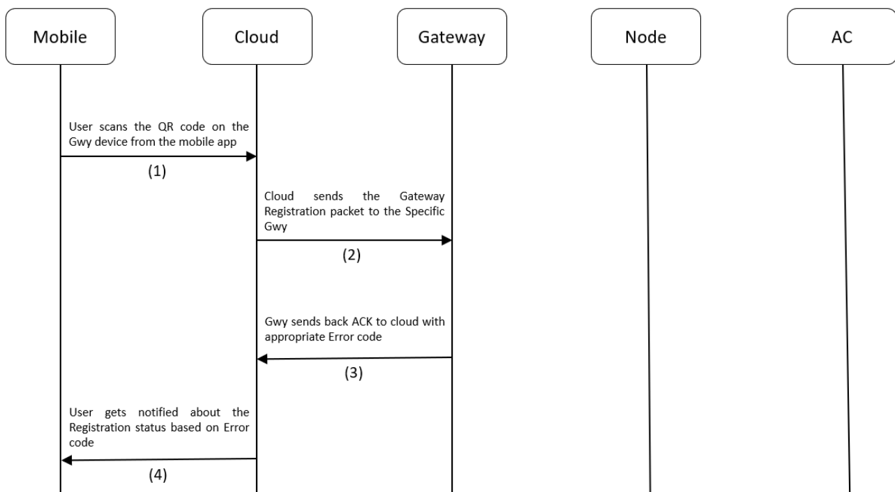
Figure 4.3 Gateway Registration process flow
