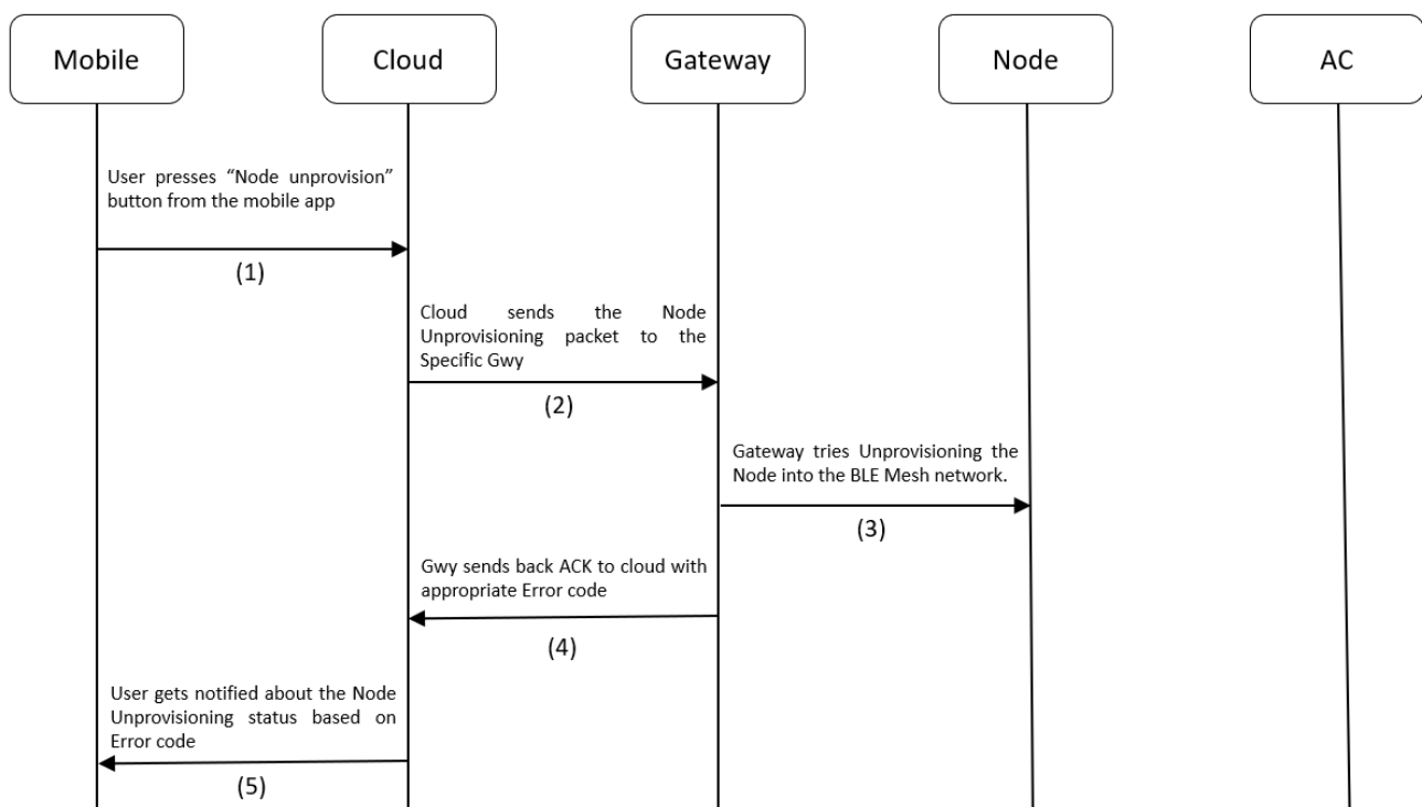
Figure 4.21 Node Unprovisioning Process flow
