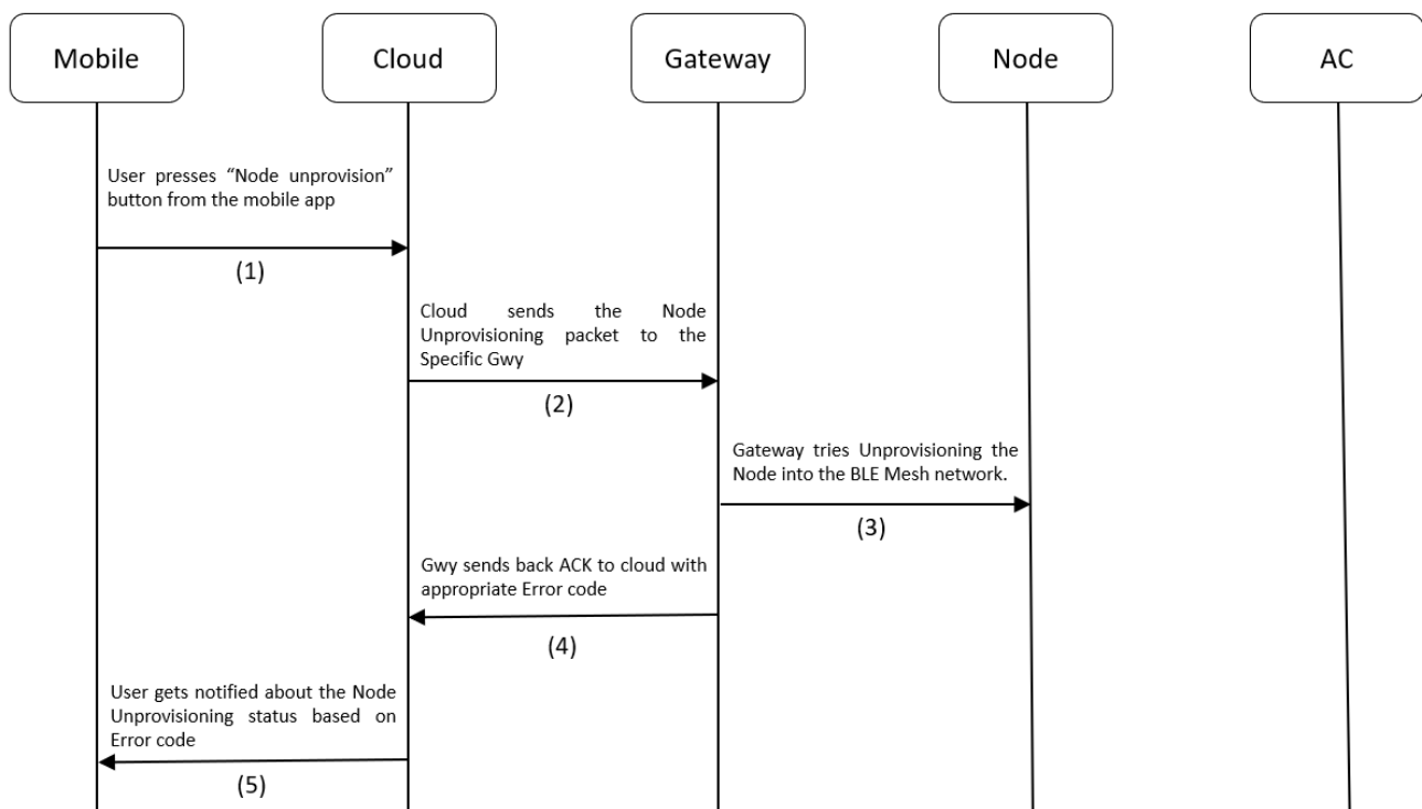
Figure 4.20 Node Unprovisioning Process flow
