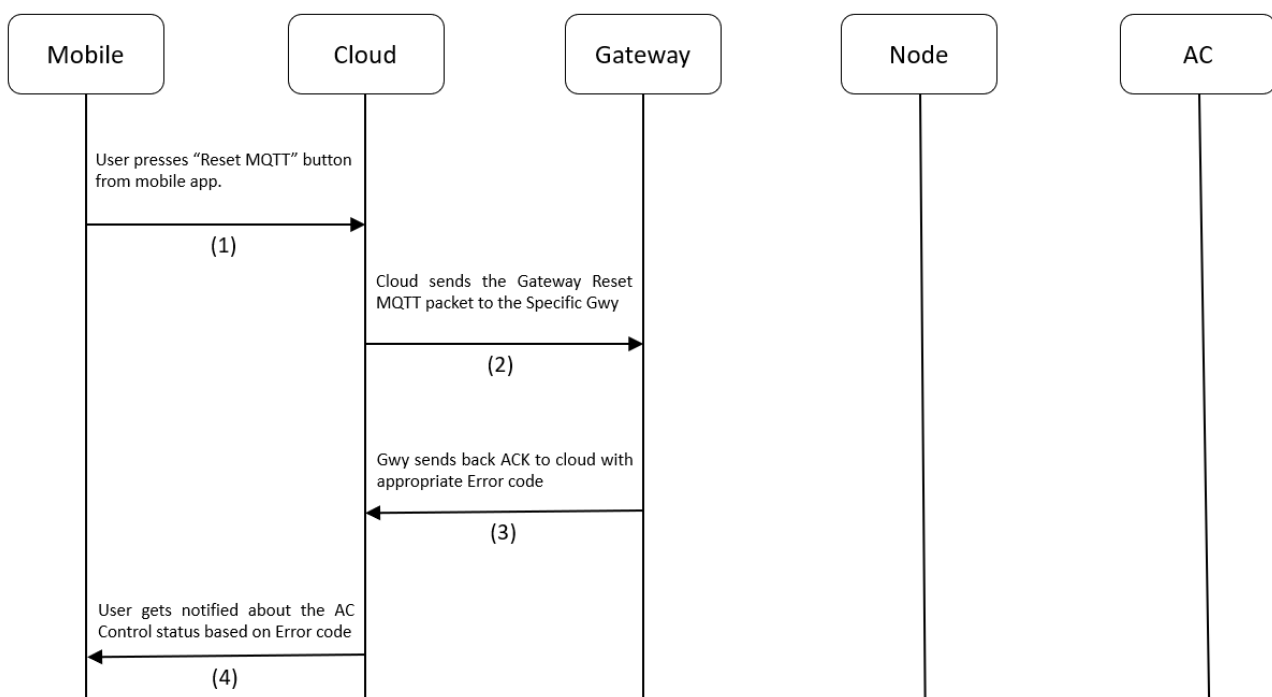
Figure 4.16 Gateway Reset MQTT Process flow
