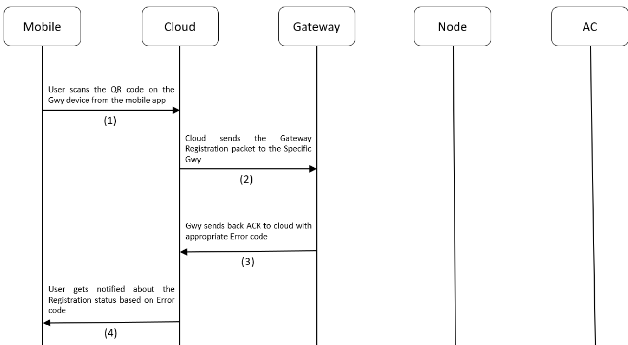
Figure 4.2 Gateway Registration process flow
