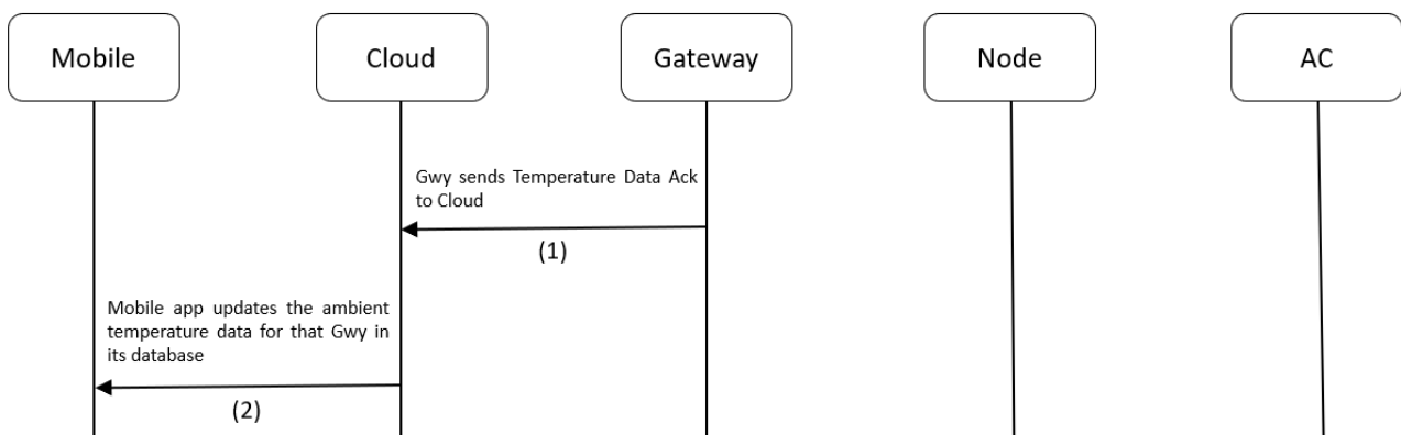
Figure 4.12 Gateway Temperature Data Process flow
