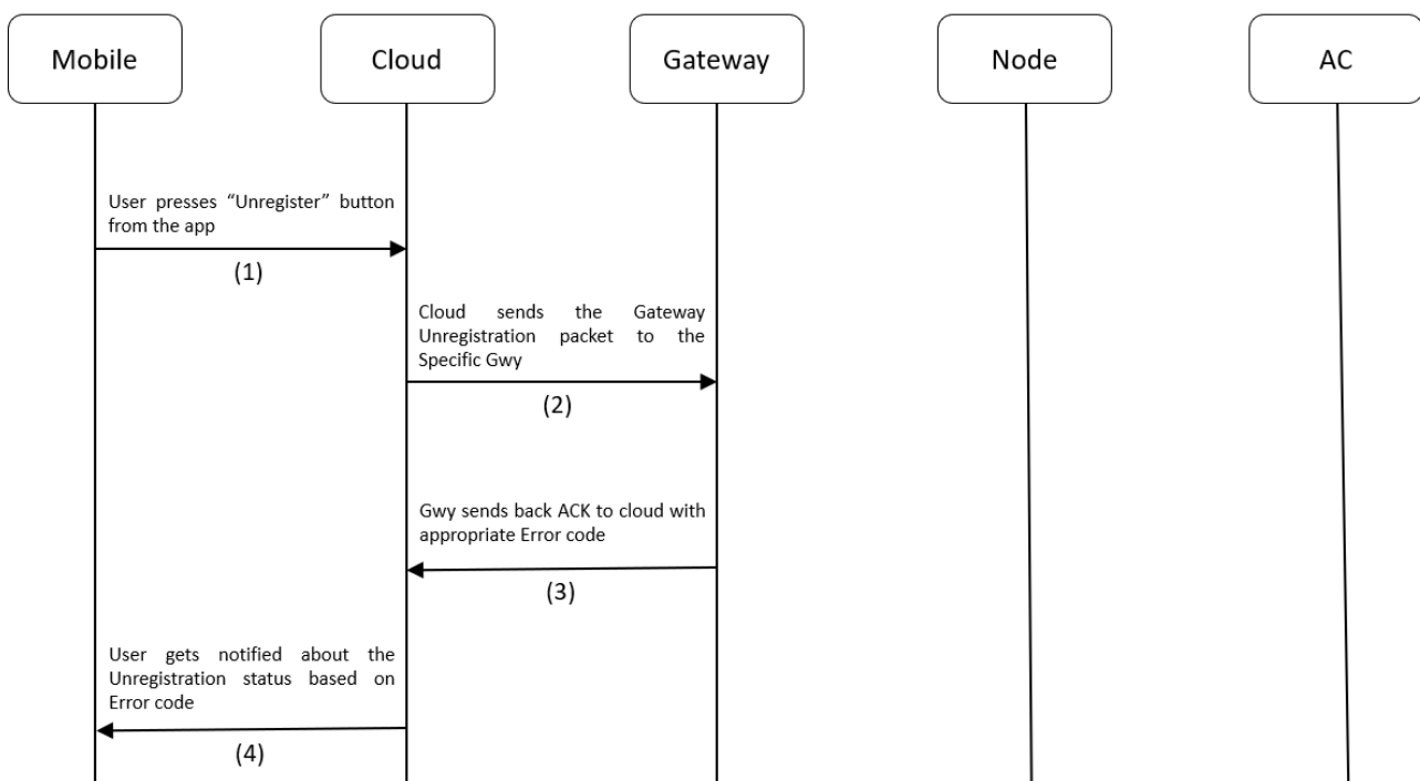
Figure 4.6 Gateway Unregistration Process Flow
