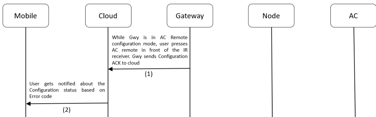
Figure 4.4 Gateway Configuration process flow
