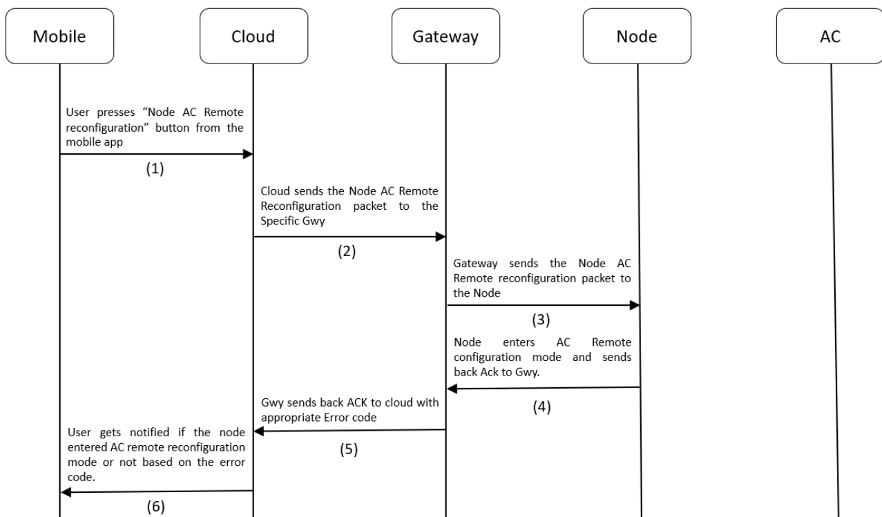
Figure 4.25 Node Reconfiguration Process flow
