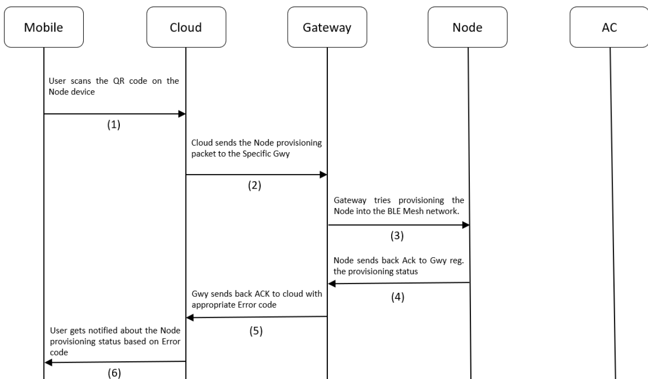
Figure 4.18 Node Provisioning Process flow
