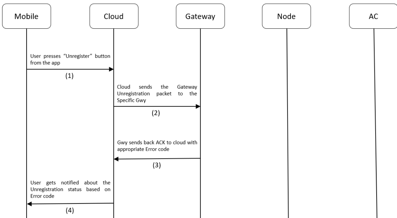
Figure 4.5 Gateway Unregistration Process flow
