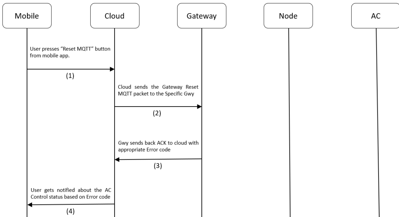
Figure 4.15 Gateway Reset MQTT Process flow
