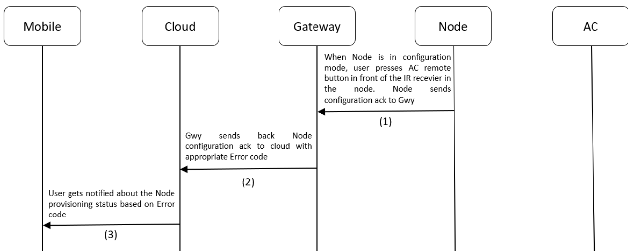
Figure 4.19 Node Configuration Process flow
