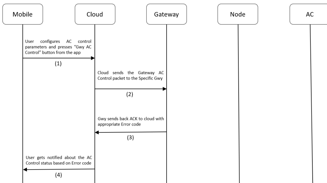
Figure 4.7 Gateway AC Control Process flow
