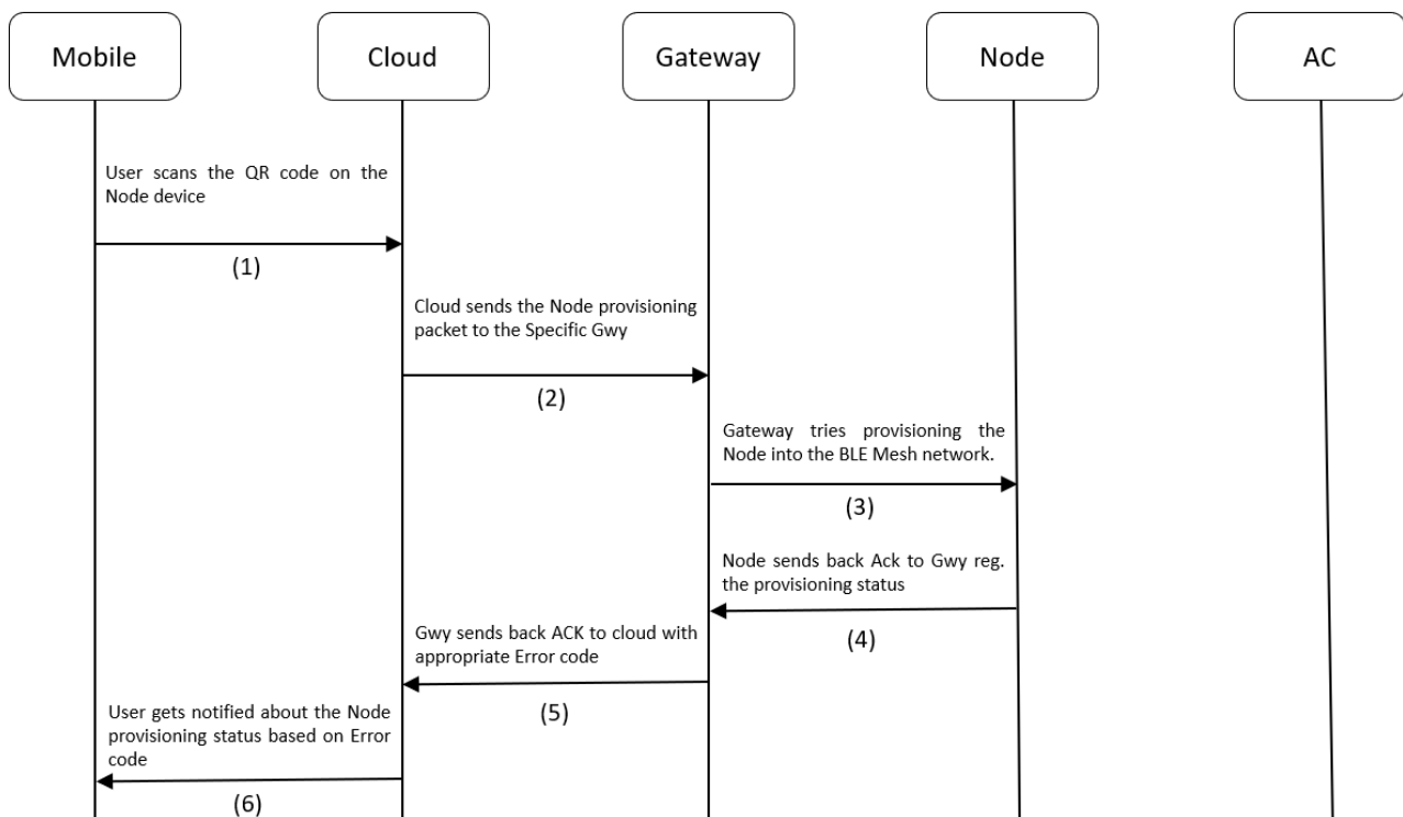
Figure 4.17 Node Provisioning Process flow
